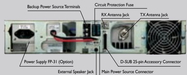
REAR PANEL
